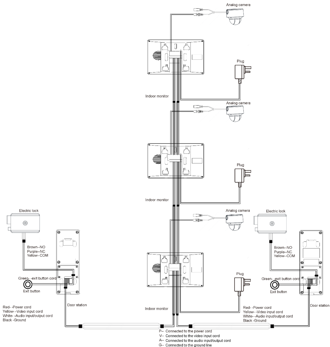
Figure 3-4 Wiring (3)
